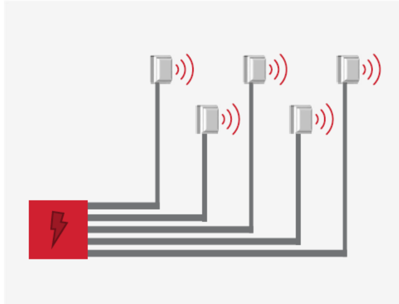
Point to Point Topology
